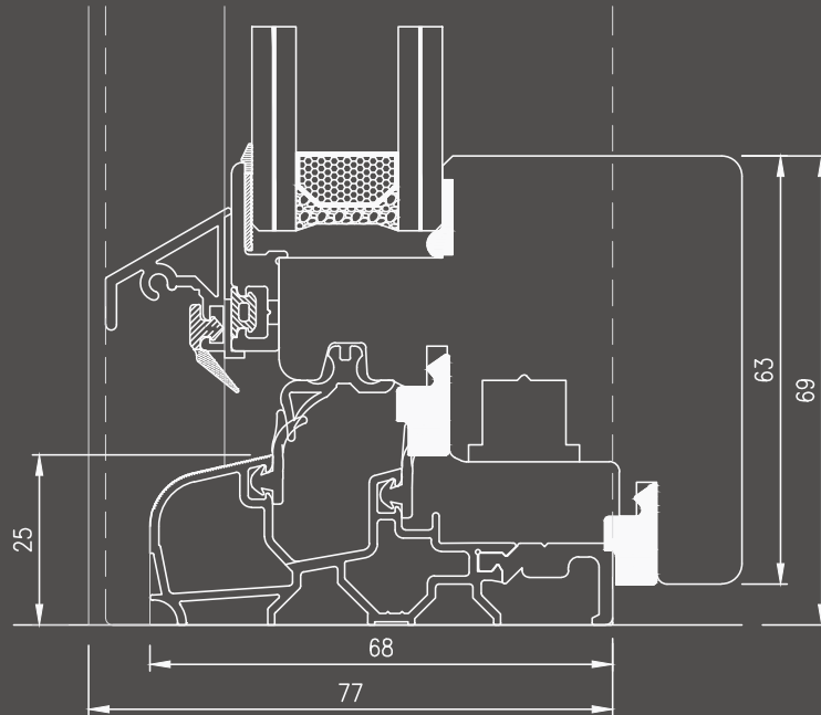
Lower node for French windows with threshold
