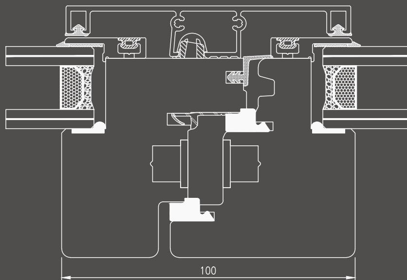
Central node of window/French window
