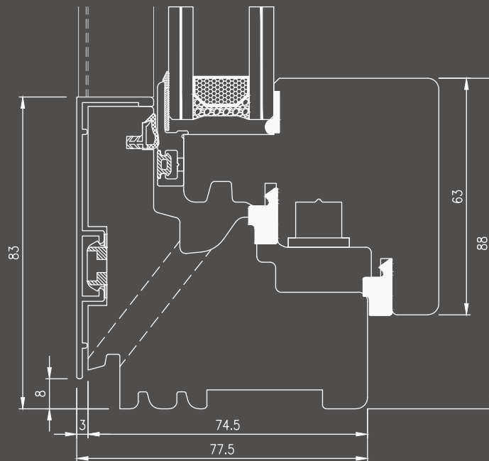
Window lower node
